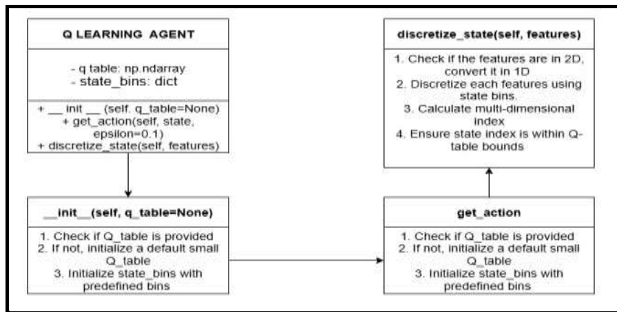
Figure 2: Diagram of QLearningAgent Class
